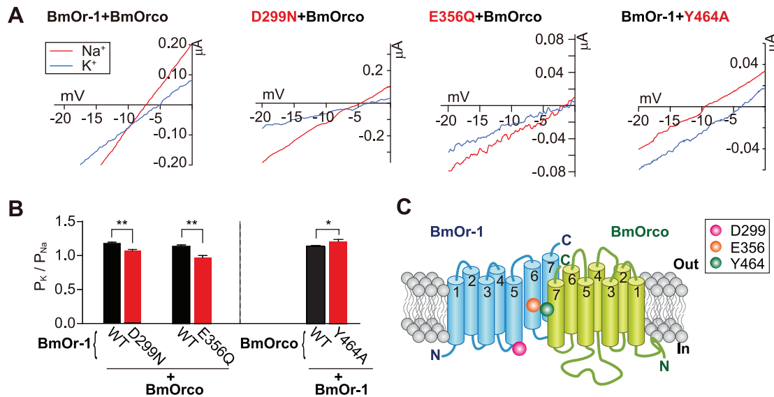
Figure 2. Mutations in BmOr-1 and BmOrco that affected ion selectivity. (A) Representative current-voltage (I-V) curves of oocytes expressing WT or mutant Or or BmOrco. Red and blue traces represent I-V curves obtained with Na + and K + solutions, respectively. (B) Summary of ion permeability ratios of the two BmOr-1 mutants (left) and the BmOrco mutants (right) that had a significant effect on ion selectivity (unpaired Student's t-test, mutant vs. WT **p<0.01; *p<0.05). Data on remaining mutants can be found in Figure S2C . Each bar represents mean ± S.E.M., n=5–8. Bombykol was applied at the concentration of 1 μM to each oocyte. (C) Schematic showing the two mutations in BmOr-1 and one mutation in BmOrco that affected ion selectivity (see also Figure S2C,S3B ). doi:10.1371/journal.pone.0032372.g002
