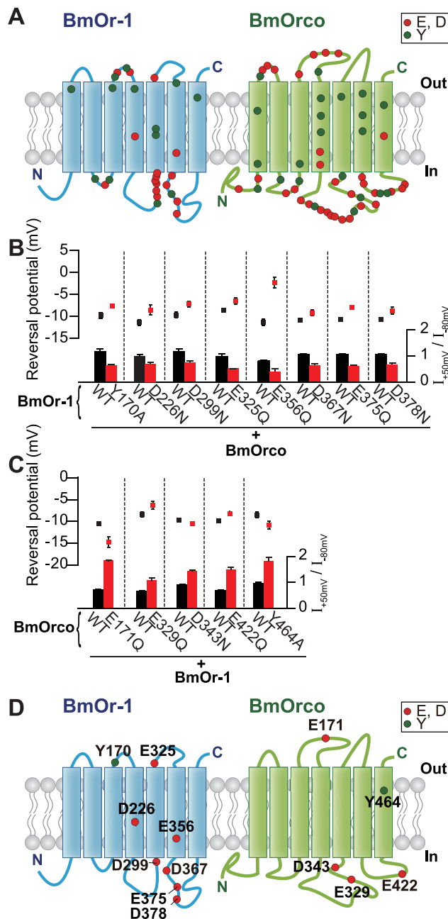
Figure 1. Mutations in BmOr-1 and BmOrco that affected reversal potential and rectification index. (A) Schematic of the location of amino acids in BmOr-1 and BmOrco that were mutated in this study. Transmembrane domains were predicted using the PHDhtm algorithm [48]. (B,C) Reversal potential (top) and rectification index (bottom) of oocytes expressing mutant BmOr-1 with wild type (WT) BmOrco (B) or WT BmOr-1 with mutant BmOrco (C). Black and red bars and symbols represent WT and mutants, respectively. Only mutants with a significant effect on both reversal potential and rectification index are depicted (unpaired Student's t-test, mutant vs. WT p < 0.05 ). Data on remaining mutants can be found in Figure S2B . Data are shown as mean \pm S.E.M., n = 8-10 . Bombykol was applied at the concentration of 1 \mu M to each oocyte. (D) Schematic showing the eight mutations in BmOr-1 and five mutations in BmOrco that affected both rectification index and reversal potential (see also Figure S2B,S3A ). doi:10.1371/journal.pone.0032372.g001
