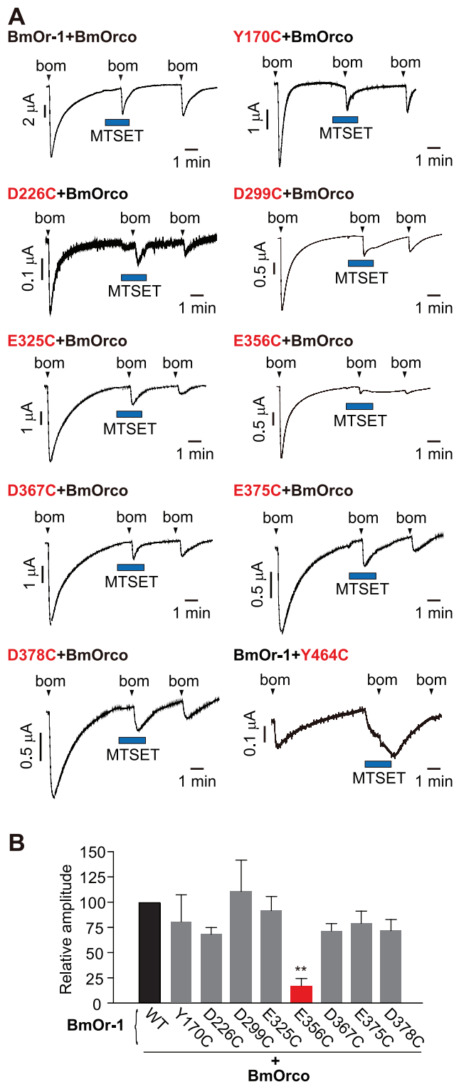
Figure 3. Effect of MTSET on ionic permeability of WT and Cys mutant BmOr-1-BmOrco complexes. (A) Representative current traces of oocytes expressing WT or mutant BmOr-1 or BmOrco. Bombykol (1 \mu M) and MTSET (2.5 mM) were applied at the time indicated by arrowheads and blue squares, respectively. (B) Summary of effects of MTSET on the bombykol response of WT (black bar) and mutant BmOr-1 (gray bars). The mutant with a significant effect on ion permeability is colored in red (unpaired Student's t-test, mutant vs. WT **p < 0.01 ). Data are shown as mean \pm S.E.M., n = 5 (see also Figure S4). doi:10.1371/journal.pone.0032372.g003
