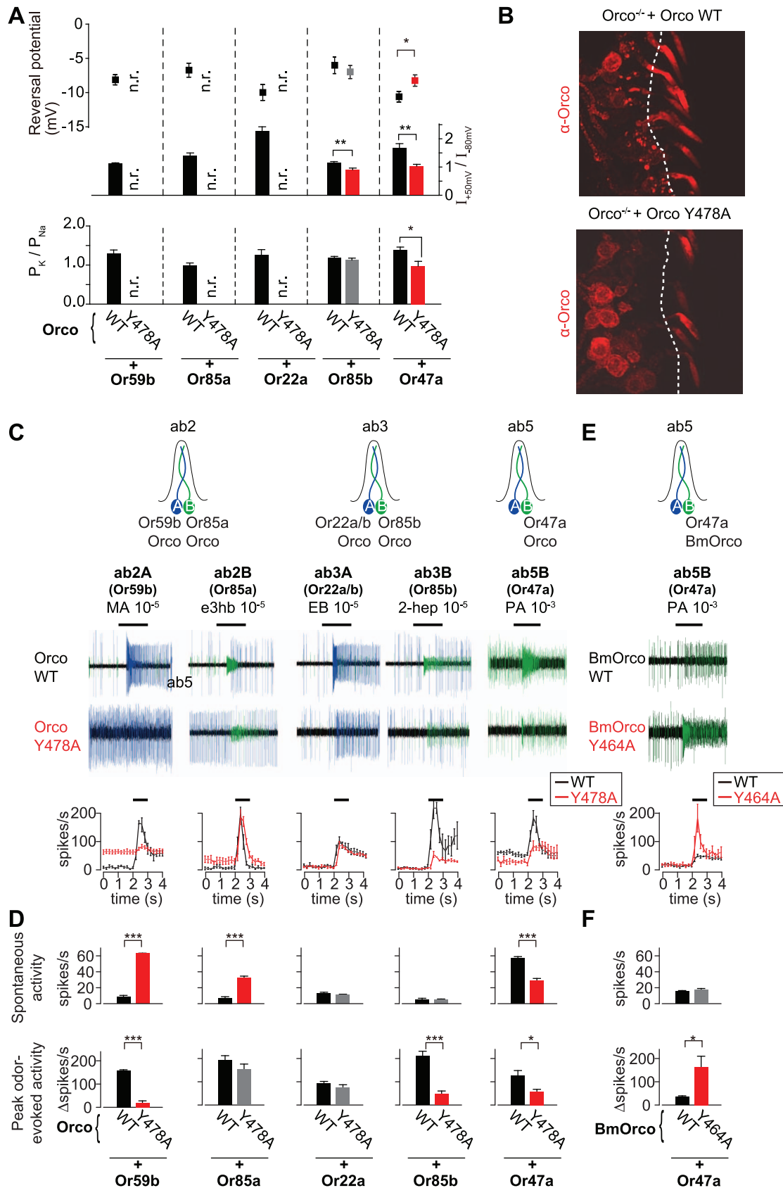
Figure 4. Effect of the Drosophila Orco Y478A mutation on Or-Orco function in heterologous cells and in Drosophila olfactory neurons. (A) Reversal potential (top), rectification index (middle), and permeability ratio (bottom) of oocytes expressing WT Drosophila Orco (black bars and symbols) or Drosophila Orco Y478A (red bars and symbols) along with WT ligand-selective Ors. Unpaired Student's t-test, mutant vs. WT,
