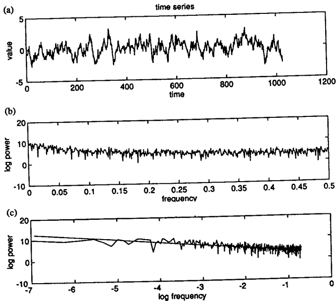
Figure 2. (a) A pseudo-red-noise time series Y of length T = 1024 ; (b) its power spectrum as a function of frequency; (c) its power spectrum as a function of log-frequency, displayed together with a fitted least-squares line.
