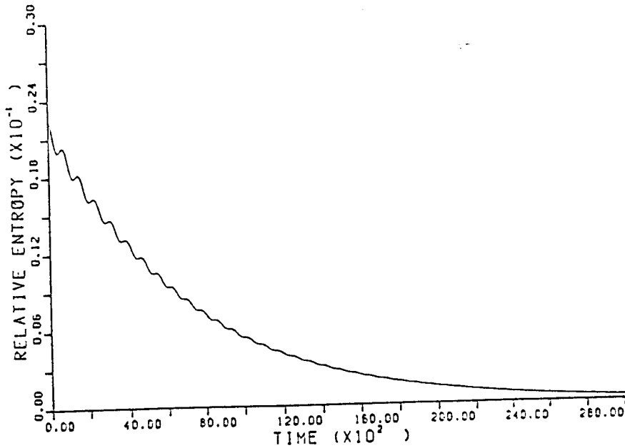
Figure 3. The relative entropy of the two distinct trajectories has damped oscillations with time far from equilibrium and is monotonically decreasing near equilibrium. The two trajectories start from (0.3, 0.3, 0.4) and (0.35, 0.35, 0.3) for p \in A^3 with a_{12} = a_{23} = a_{31} = \frac{1}{2} , where k_1 = 20 and k_2 = 2.1 .
