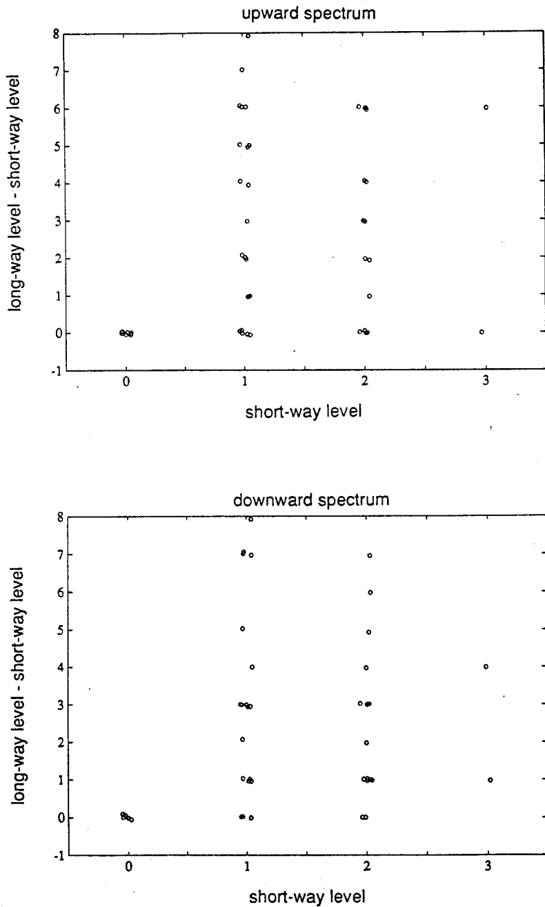
Figure 4. Spectra of a single simulation of the cascade model with parameters S = 48 and d = 5.8723 identical with those of the Sonora Desert web in Figure 3. (a) Upward spectrum. (b) Downward spectrum. Each data point has exactly integer coordinates, but has been perturbed by a small random amount to render coincident points visible. Each symbol represents one species.
