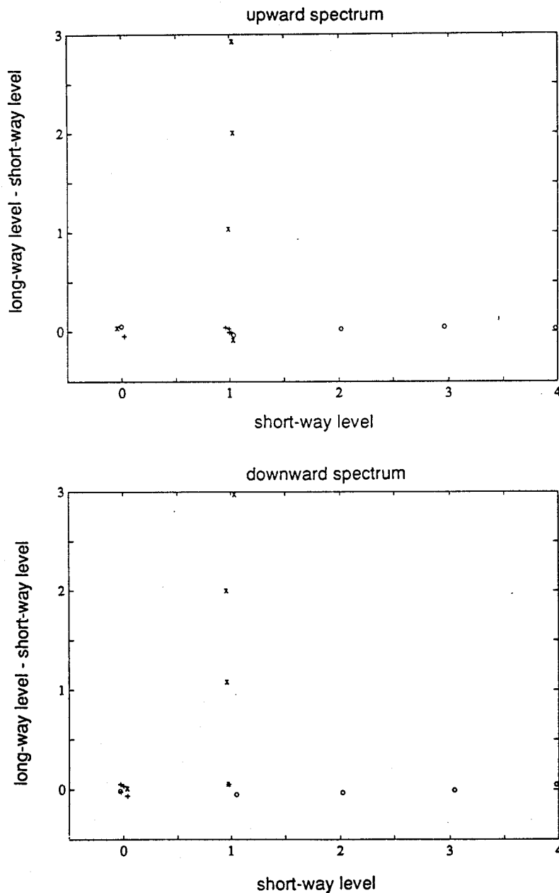
Figure 2. Spectra of three hypothetical webs. (a) Upward spectra. (b) Downward spectra. Symbols: O = chain; + = bush; X = vine. Each data point has exactly integer coordinates, but has been perturbed by a small random amount to render coincident points visible. Each symbol represents one species.
