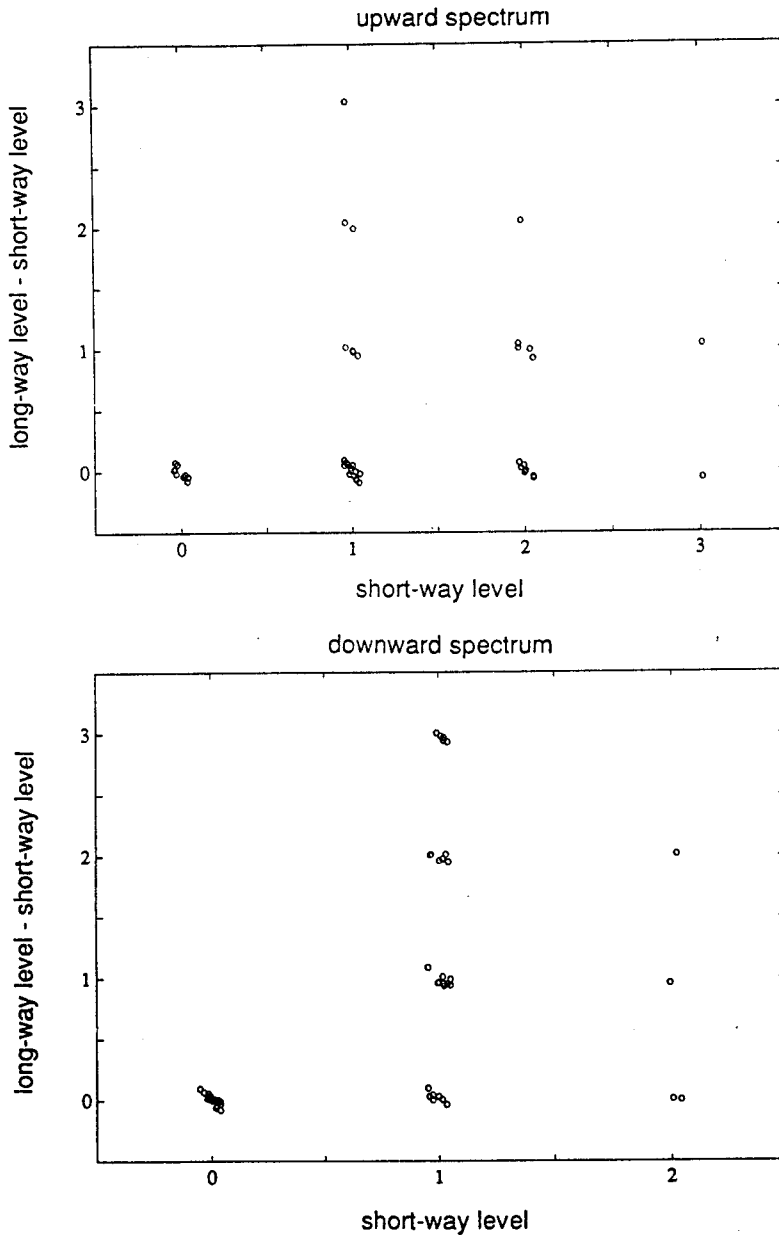
Figure 3. Spectra of the food web of the Sonora Desert, Arizona, according to Howes (1954) as edited by Briand (Cohen et al. , 1990, web 99, pp. 270–1). (a) Upward spectrum. (b) Downward spectrum. Each data point has exactly integer coordinates, but has been perturbed by a small random amount to render coincident points visible. Each symbol represents one species.
